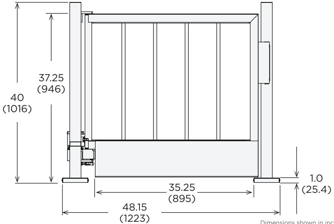
Dimensions shown in inches (mm).
